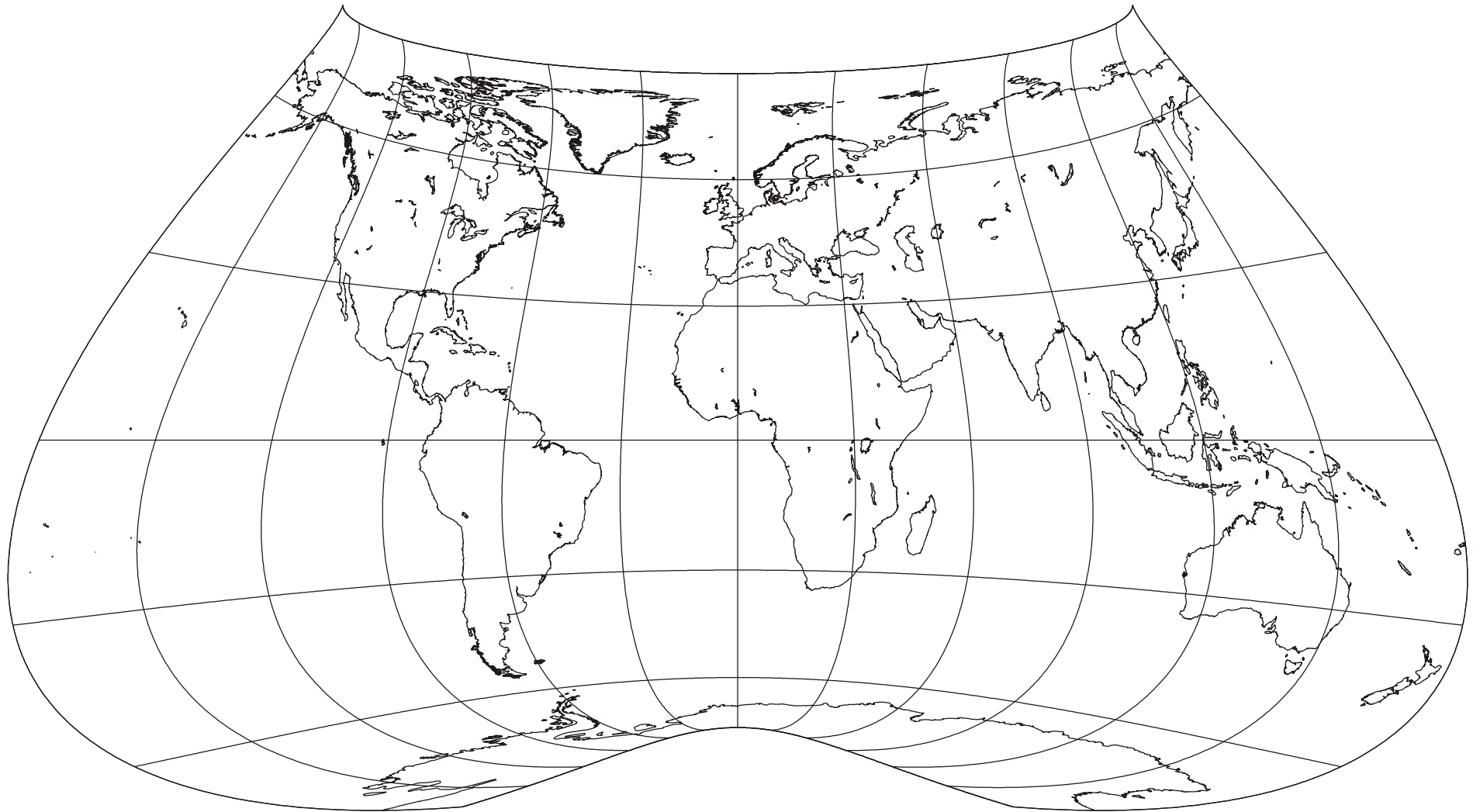
Low-error Polyconic; (with straight equator and symmetry about the central meridian); Neither Conformal or Equal-area; Frank Canters; 1989, 2002
