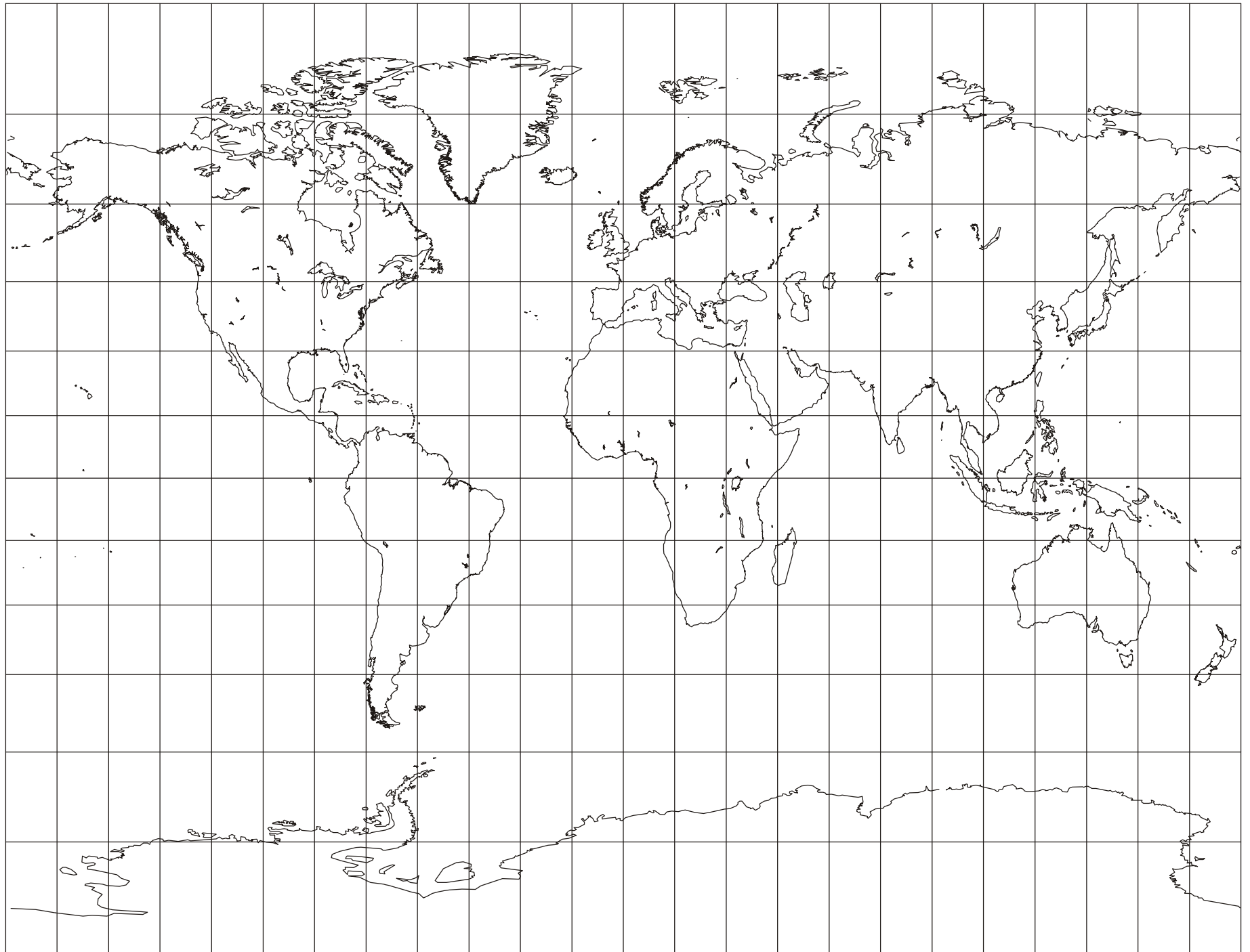
Gall Stereographic; Cylindrical; Neither Conformal or Equal-area; Standard Parallels = 45 Deg. N/S; James Gall; 1855
